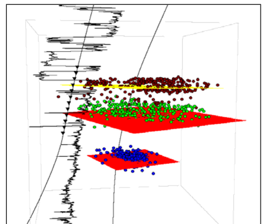
Visualization of Microseismic Events
