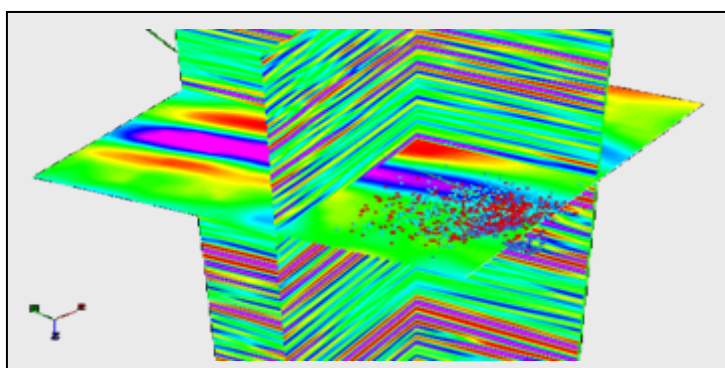
Composite plot of Microseismic and 3D data
