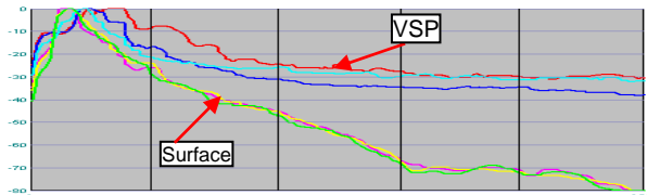
Spectra Comparison Before Processing
