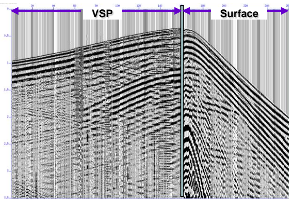
VSP and Surface Shot Gather
