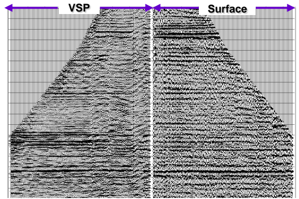
VSP and Surface Seismic Gather After NMO
