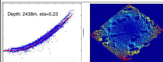
Residual time after isotropic processing
