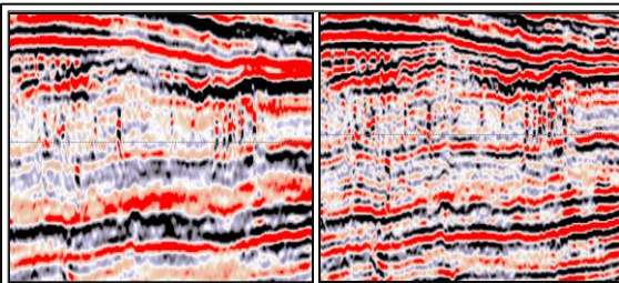
Comparison of VSP-driven Q compensation
