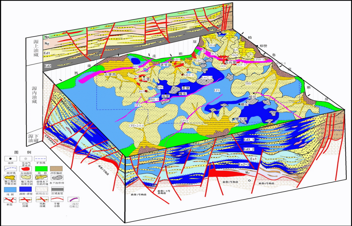
Deposition model, stratigraphic traps, and reservoir development model
