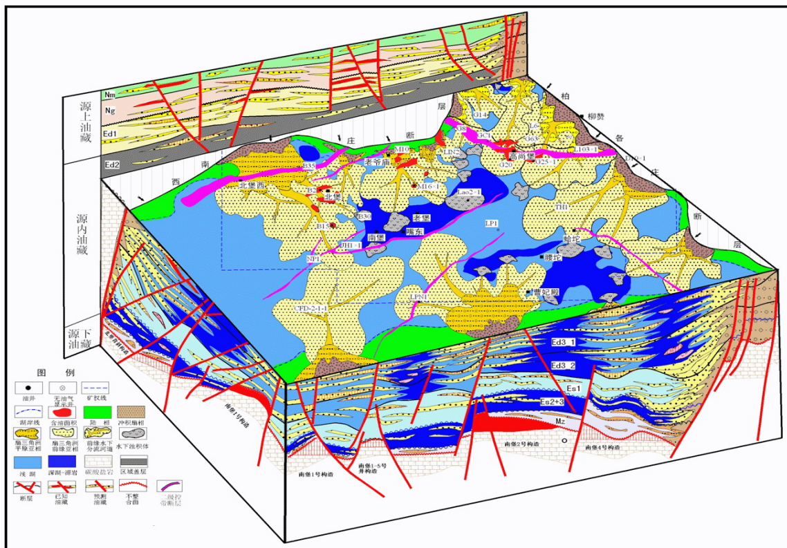
Deposition model, stratigraphic traps, and reservoir development model
