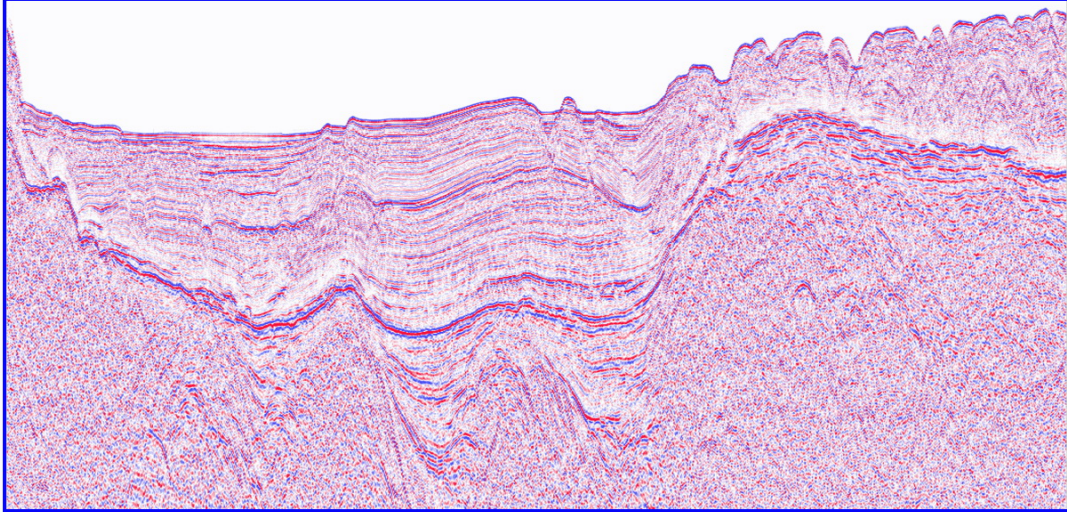
2D marine seismic section in South China Sea
