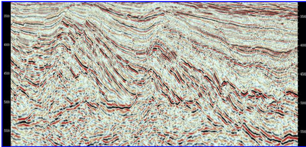
3D seismic section in South China Sea
