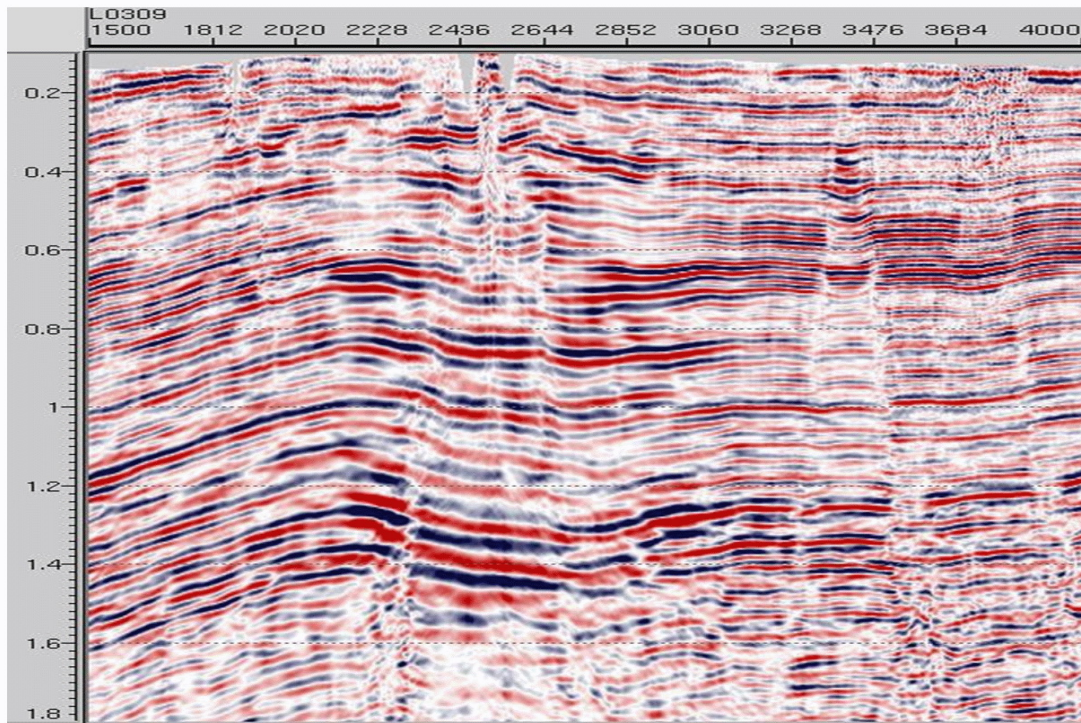
P-wave pre-stack time migration
