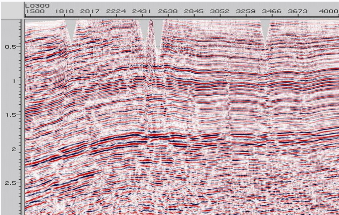
C-wave pre-stack time migration
