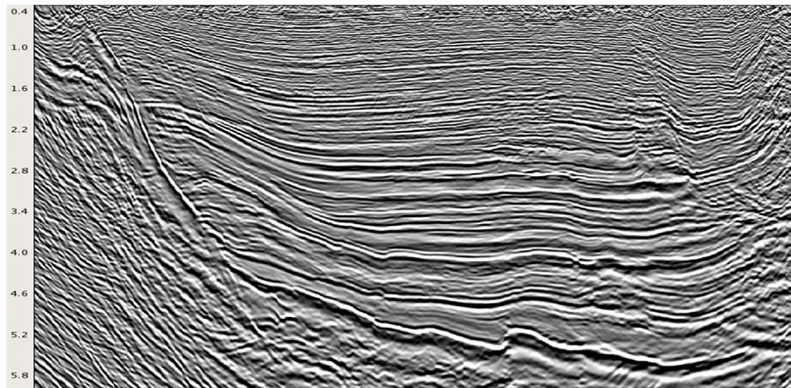
One-way wave equation PSDM section
