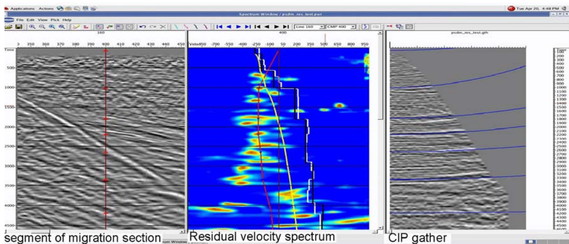
Residual velocity analysis for PSDM
