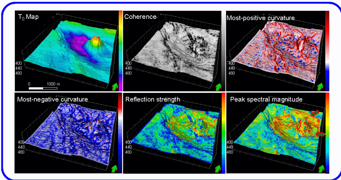
Prediction of igneous rock distribution, volcanic crater, and fracture development with multi-attributes
