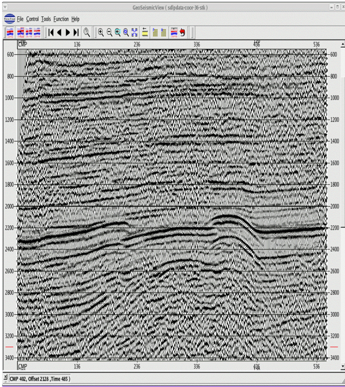
Stack section after Torro-static corrections
