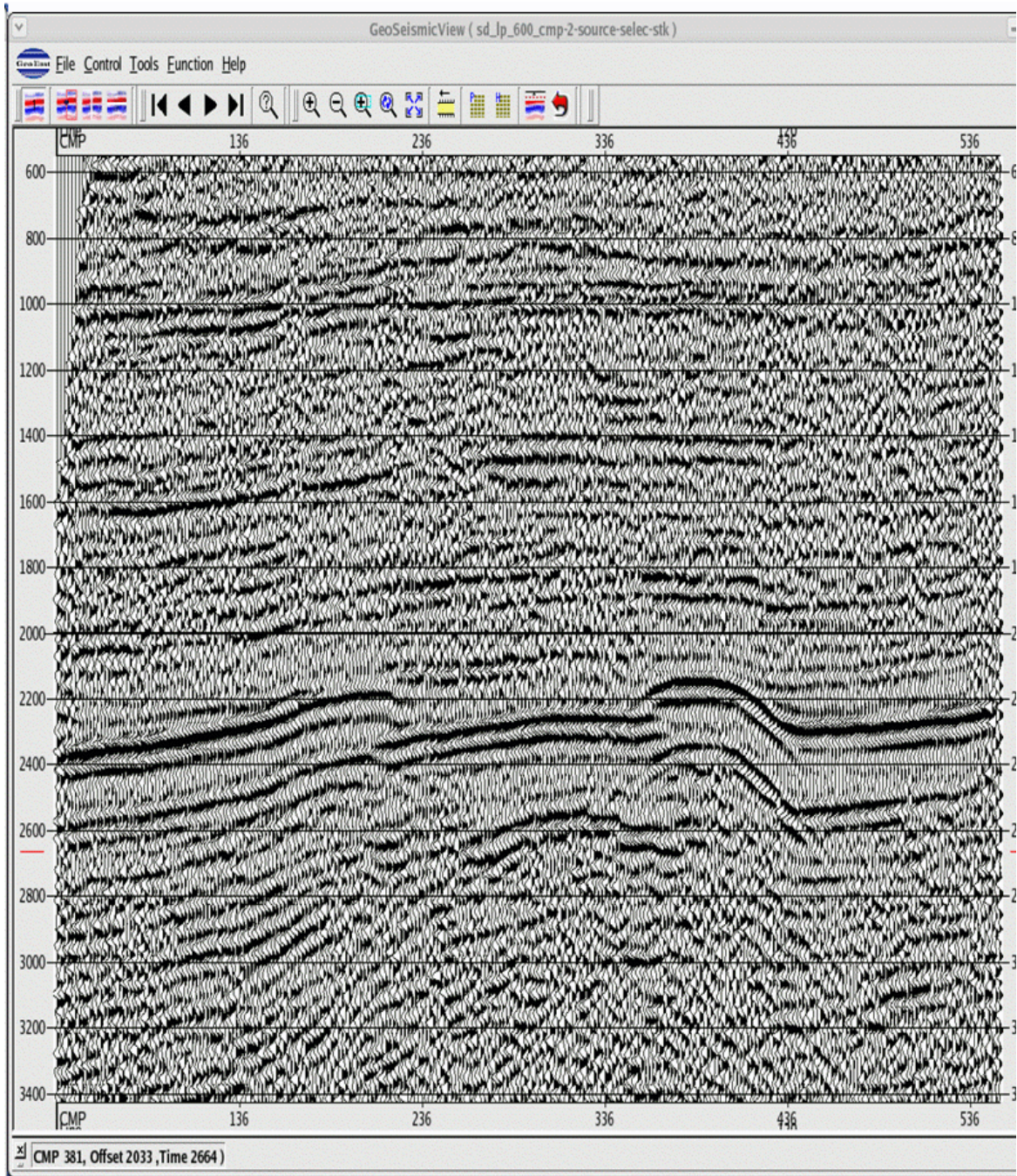
Stack section after elevation static corrections
