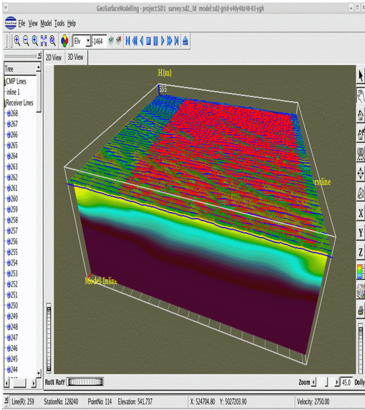
Near-surface velocity model from Tomo-inversion
