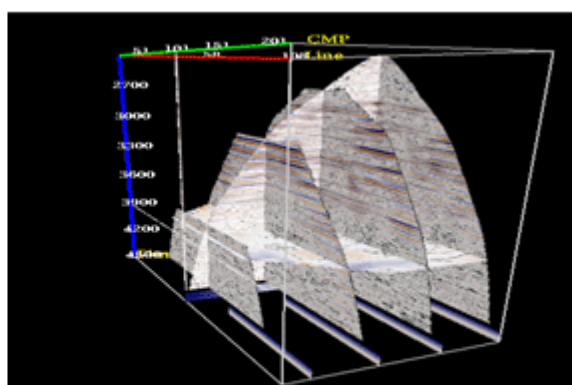
3DV of migrated 3D VSP data
