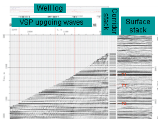
Calibration of zero offset VSP section and CMP section
