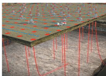
multiple wells DAS VSP and surface seismic joint acquisition
