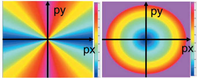
Azimuth (left) and take-off angle (right) in 3D tau-p domain
