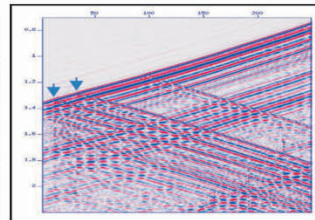
Multiples identification and attenuation
