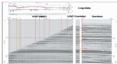
Calibration seismic data with VSP and logging
