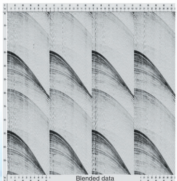
Deblending of blended land and streamer data Top: blended data and deblended land primary shot Bottom: blended data and deblended streamer primary shot
