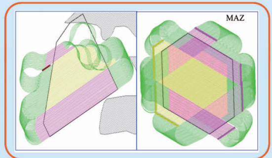
Streamer acquisition design
