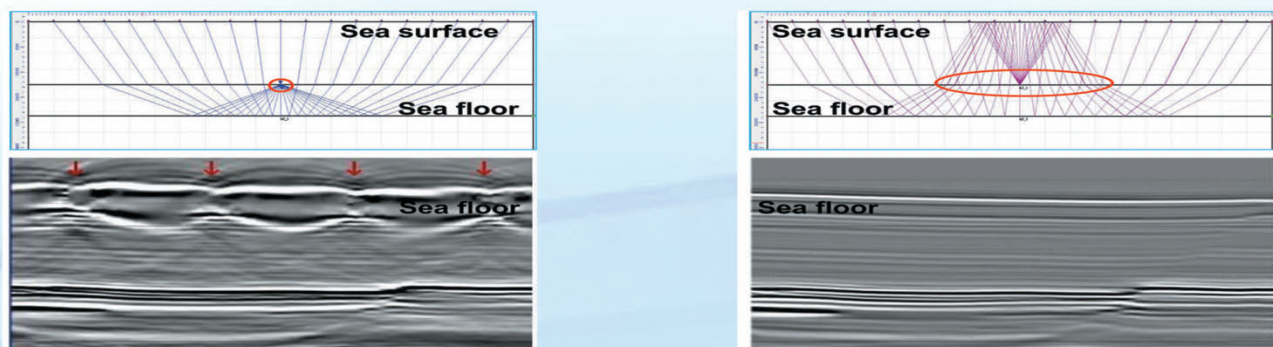
Illumination of up-going wave PSTM (left) vs. down-going wave mirror PSTM (right)
