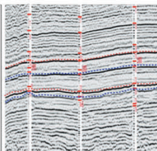
Calibration seismic data with VSP and logging
