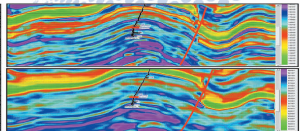
Comparison of wave impedance inversion between walkaway VSP (above) and surface seismic (below)
