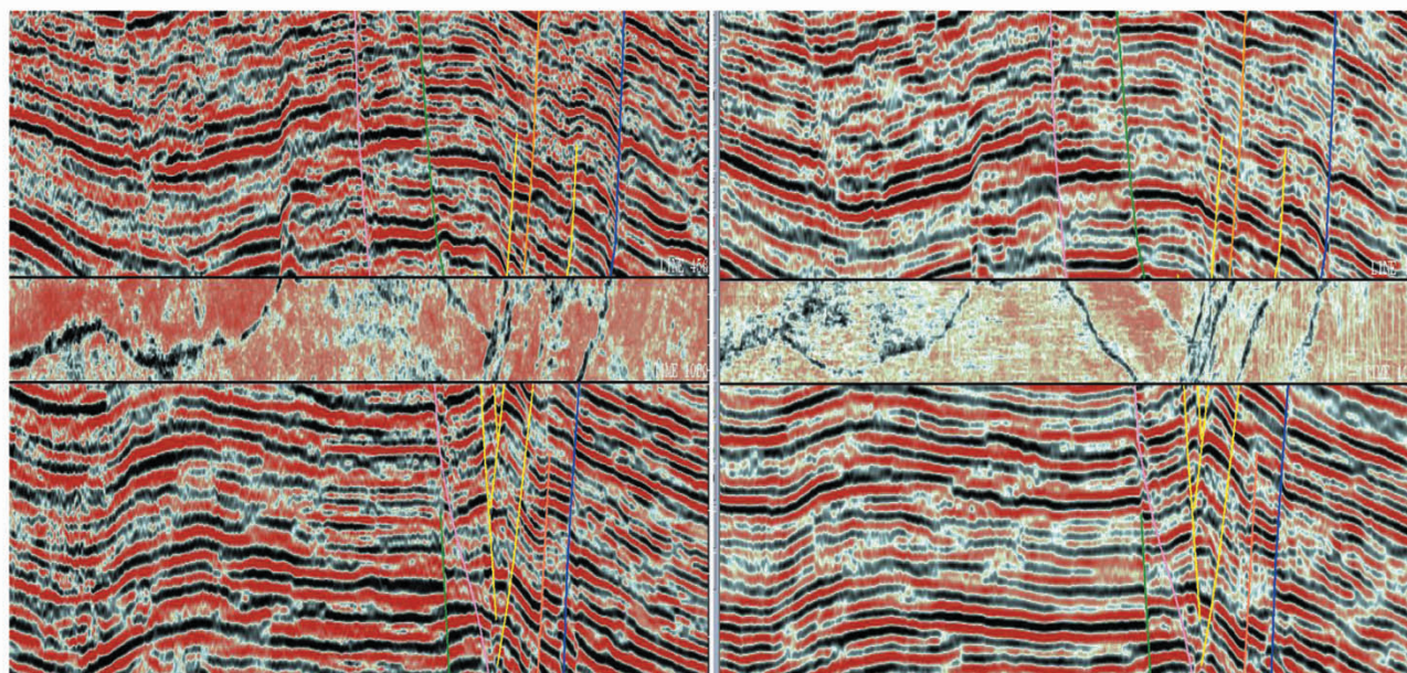
Migration section (Hydrophone)
