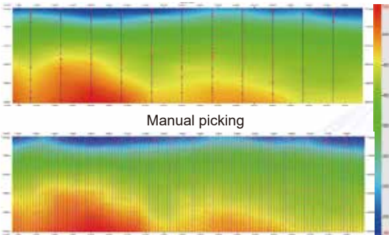
DL picking
