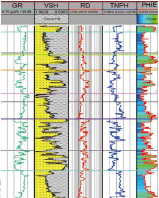
Petrophysical analysis
