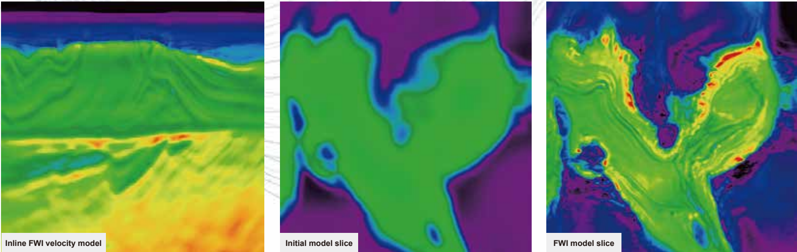
Geological modeling
